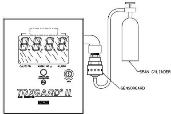
Figure 3-15. Span Set-up
