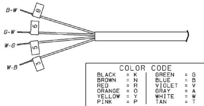
Figure 1-9. Oxygen Remote Sensor Cable
