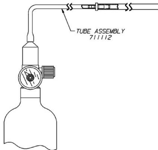
Figure 3-7. Calibration Tubing Set-up
