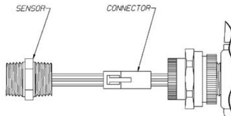
Figure 5-5. Combustible Three-Pin Connector
