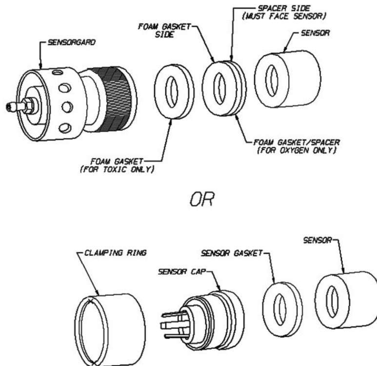
Figure 5-3. Cap Location for Toxic Gas or Oxygen General-purpose Model
