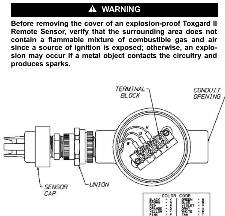
Figure 1-8. Combustible Remote Sensor
