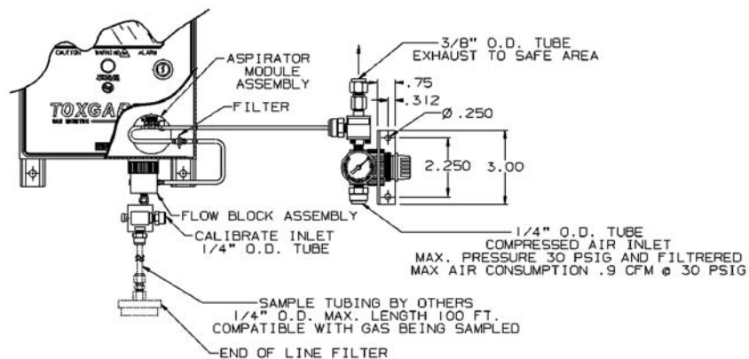
Figure 3-19. Typical Air Aspirator Version Installation
