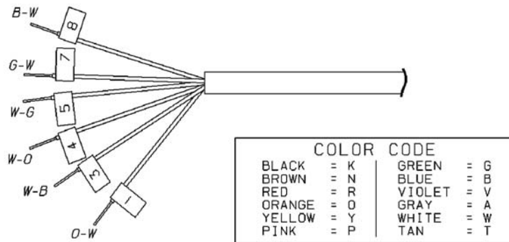
Figure 1-11. Toxic Gas Remote Sensor Cable
