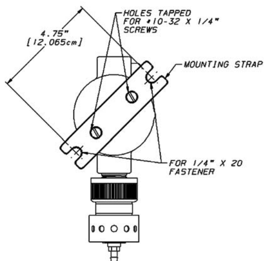
Figure 1-5. Remote Sensor Mounting Method
