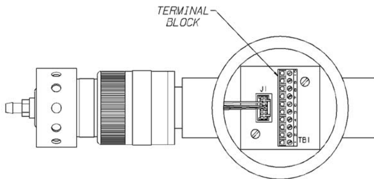
Figure 1-10. Oxygen and Toxic Remote Sensor
